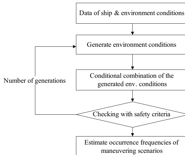
Figure 3.14: Calculation procedure
