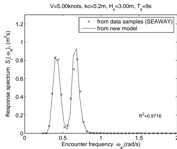
Figure 5.13: Comparison between the theoretical ship response calculations (SEAWAY) and the results from the parametric model (b)
