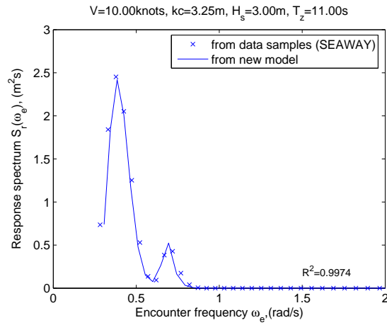
Figure 5.12: Comparison between the theoretical ship response calculations (SEAWAY) and the results from the parametric model (a)
