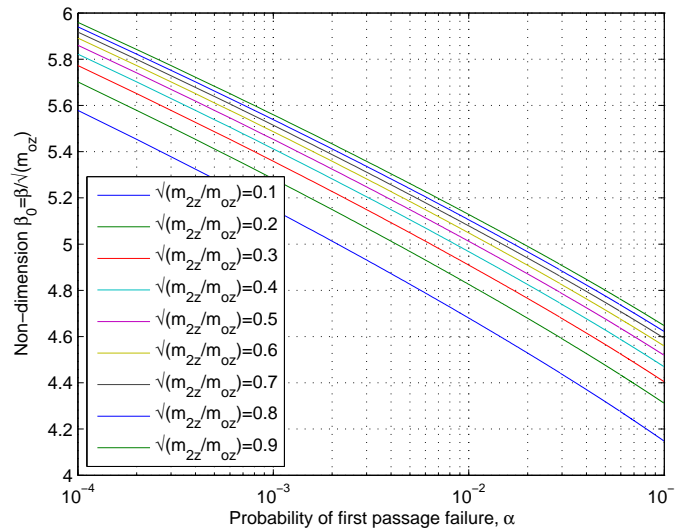
Figure 5.4: Non-dimensional \beta_0 vs. \alpha for T_h = 10 hours
