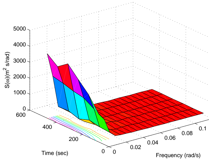
Figure 4.6: Time-dependent spectral density function of the response ensemble (at Paprotno Mielin bend part)
