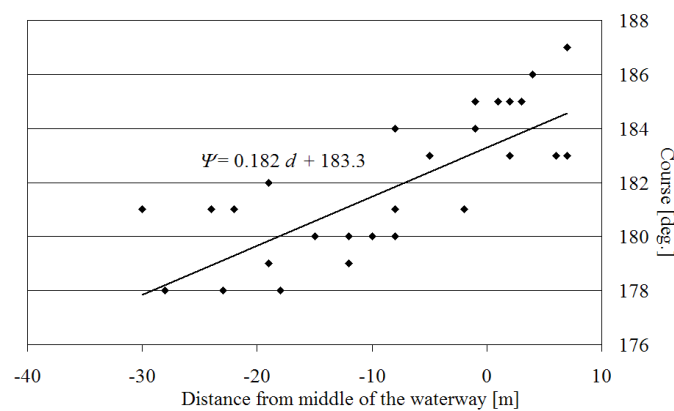
Figure 3.3: Linear correlation between distance from the waterway center and ship course for one investigated simulation trial (Guema, 2005)
